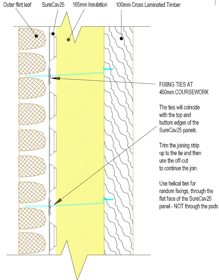
TIMBER-FRAME TIE WITH SURECAV25
